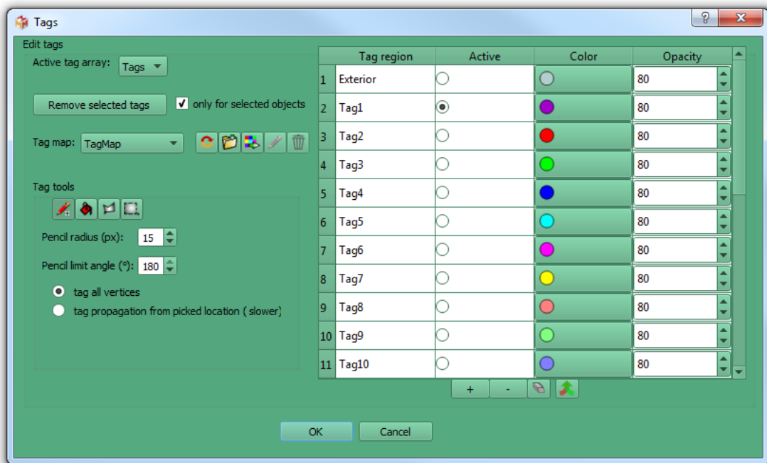
Figure 4.3: Tags window.
